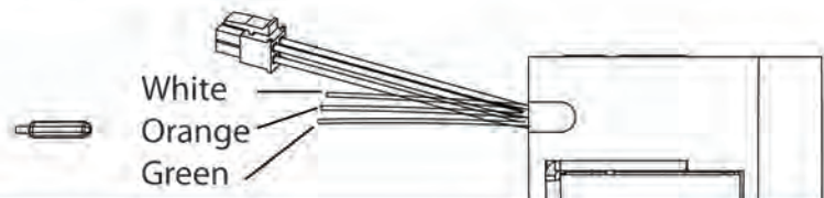
DIAGRAM 3: LATCHBOLT MONITOR
