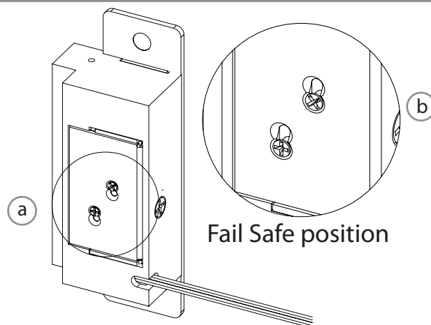
DIAGRAM 4: FAIL SAFE CONVERSION
