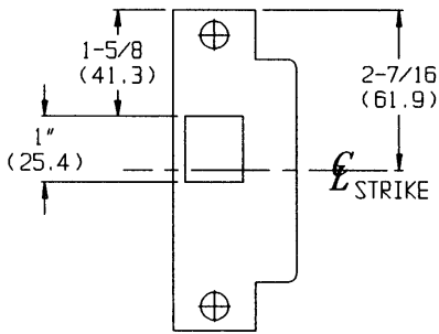
STRIKE DETAIL
