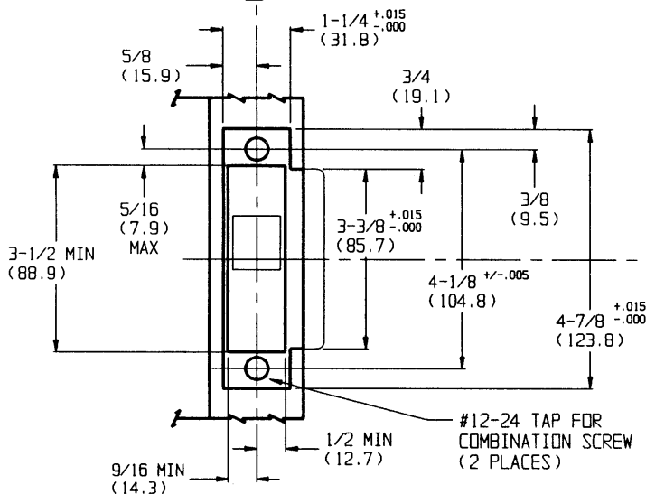
FRAME DETAIL
