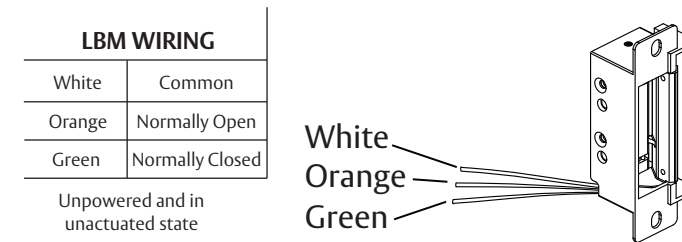
Figure 2: Latchbolt Monitor
