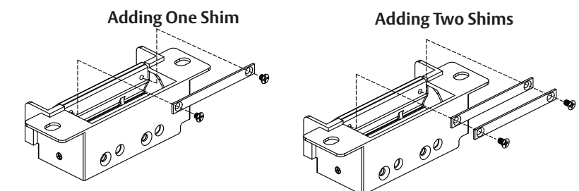
Figure 6: Horizontal Adjustment
