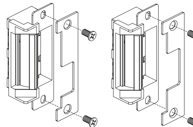
Figure 5: Faceplate Options
