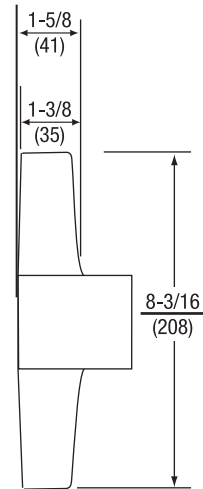
Cover Detail
